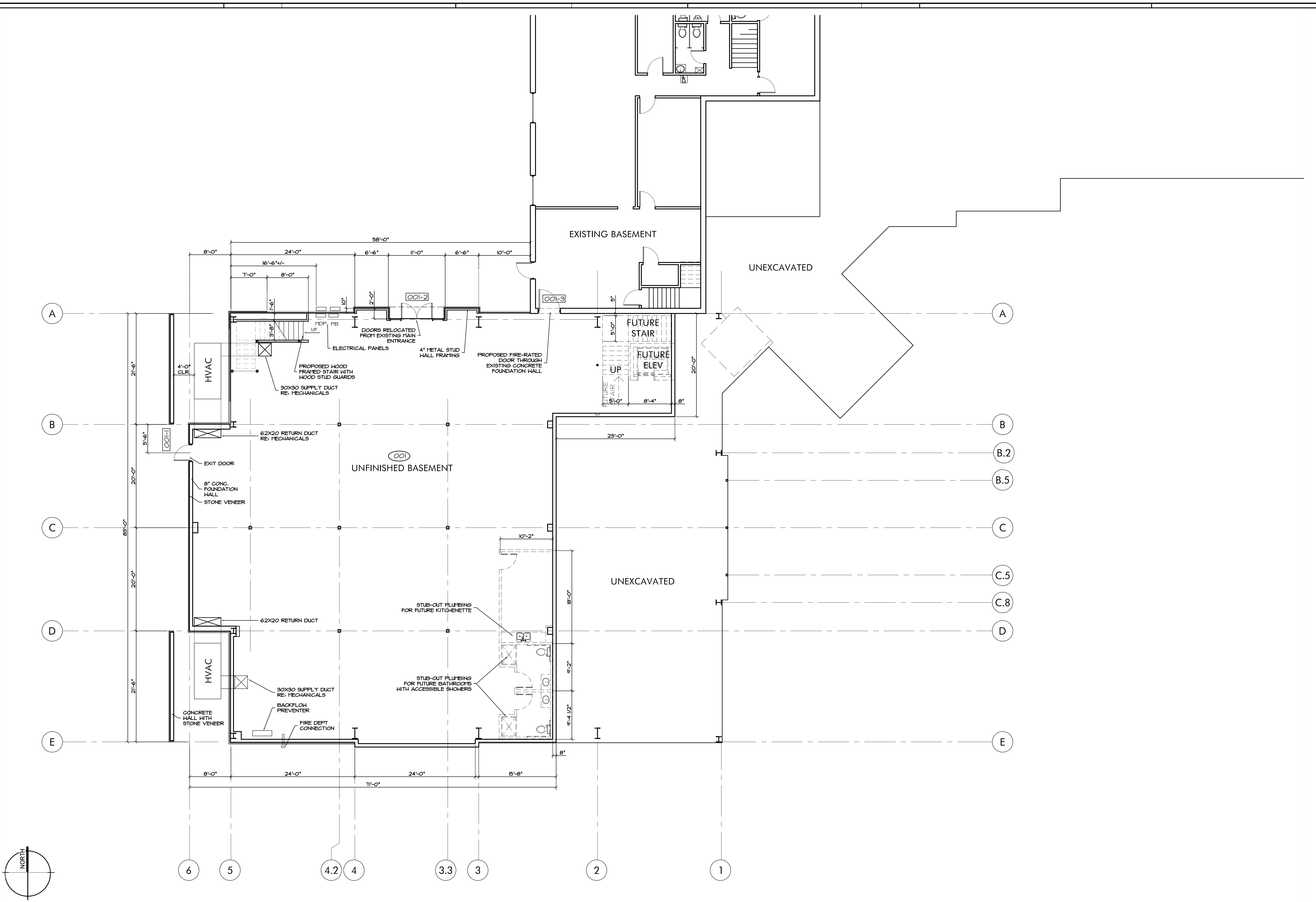
1 BASEMENT FLOOR PLAN 1/8" = 1'-0"
